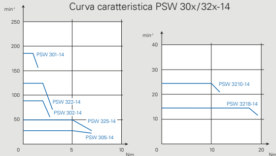
Curva caratteristica PSW 30x/32x-14
